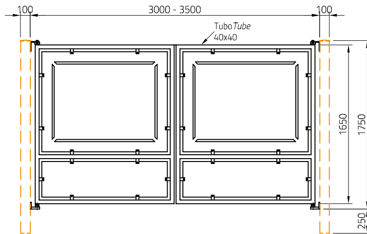
Cancello Carrabile | Driveway gate LASER-CB3017Z | LASER-CB3517Z
